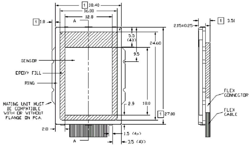
Figure 2 Sensor dimensions
